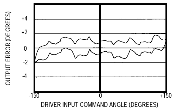
Fig. 4 Phaser error characteristic
