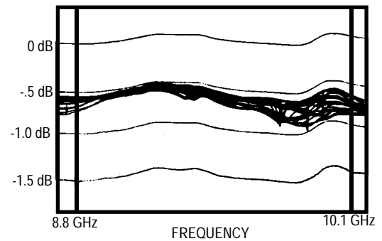
Fig. 2 Phaser insertion loss
