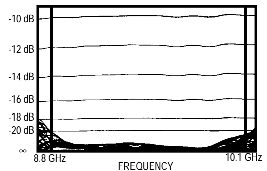
Fig. 3 Phaser return loss
